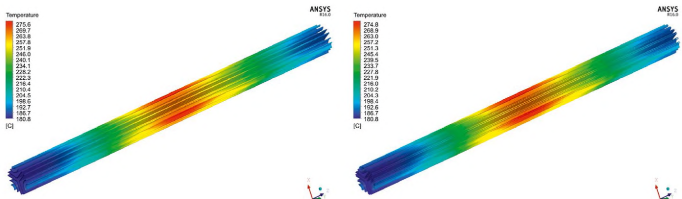
Fig. 11. The maximum temperature of the fuel and cladding
