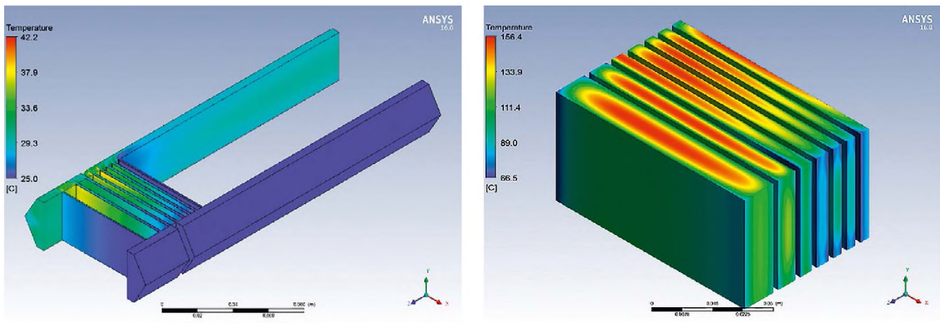
Fig. 6. NGT's coolant temperature distribution (left) and the temperature of the NGT's plates
