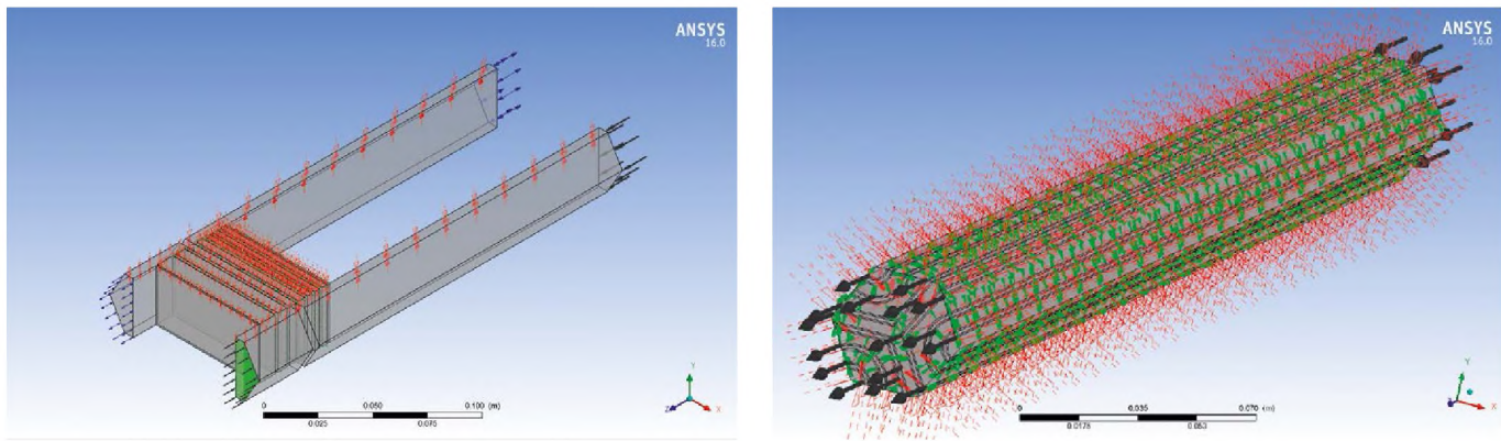
Fig. 5. NGT and FA models
