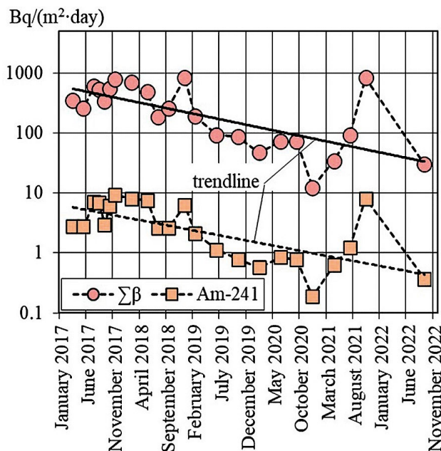
Fig. 6. Deposition density of \Sigma\beta and ^{241}\text{Am} in room 210/7 in 2017–2022
